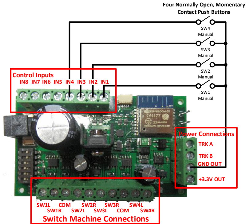
Figure 5. Connection Diagram for Manual Push Buttons
