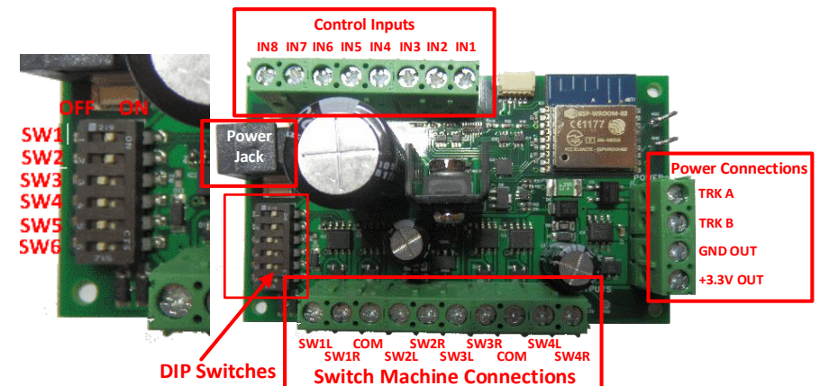
Figure 1 WFS-46 Connections
