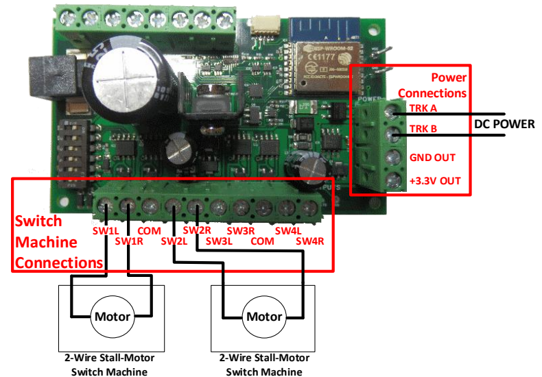
Figure 4. Connection Diagram for Stall Motor Switch Machines
