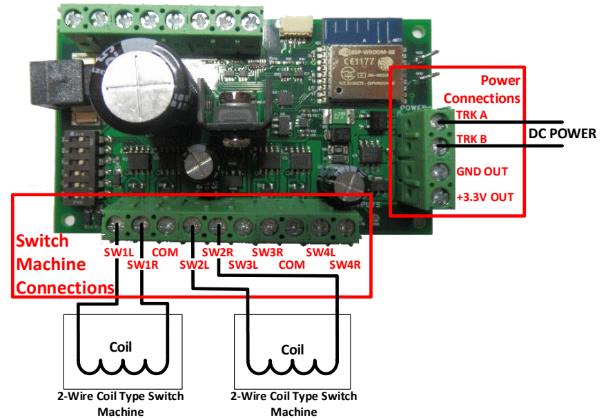
Figure 3. Connection Diagram for 2-Wire Coil Type Switch Machines
