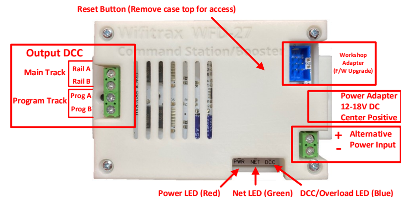
Figure 1. WFD-27E Connections
