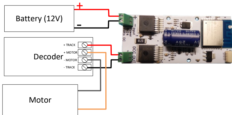
Figure 2. Connections to the WDMI-27
