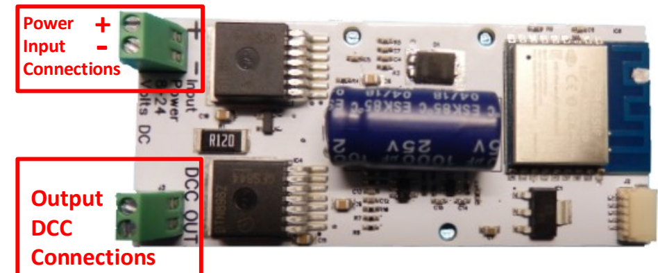
Figure 1. WDMI-27 Connections
